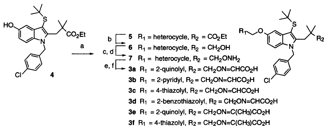
Scheme 1. Reagents and conditions: (a) chloromethylheterocycle, \text{K}_2\text{CO}_3 , DMF, 60^\circ\text{C} ; (b) \text{NaBH}_4 , \text{CaCl}_2 , THF, EtOH, 0^\circ\text{C} to rt; (c) PhNOH, \text{Ph}_3\text{P} , DIAD, THF; (d) \text{H}_2\text{NNH}_2 , EtOH, reflux; (e) \text{RCOCO}_2\text{H} , AcOH, THF, \text{H}_2\text{O} ; (f) NaOH, dioxane, MeOH, rt.
