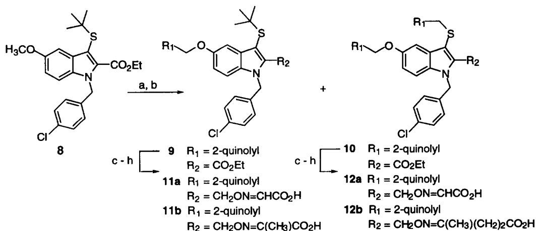
Scheme 2. Reagents and conditions: (a) \text{AlCl}_3 , t -BuSH, \text{CH}_2\text{Cl}_2 , 0^\circ\text{C} , (91%); (b) 2-chloromethylquinoline, \text{K}_2\text{CO}_3 , DMF, rt, 9 (32%) and 10 (50%); (c) NaOH, dioxane, MeOH, rt; (d) \text{ClCO}_2\text{Et} , \text{Et}_3\text{N} , THF, -15^\circ\text{C} , then \text{NaBH}_4 , MeOH, 0^\circ\text{C} ; (e) PhNOH, \text{Ph}_3\text{P} , DEAD, THF; (f) \text{H}_2\text{NNH}_2 , dioxane, EtOH, reflux; (g) \text{RCOCO}_2\text{Et} , AcOH, MeOH, dioxane; (h) NaOH, dioxane, MeOH, rt, overall yield (c–h): 11a (21%), 11b (73%), 12a (53%), and 12b (66%).
