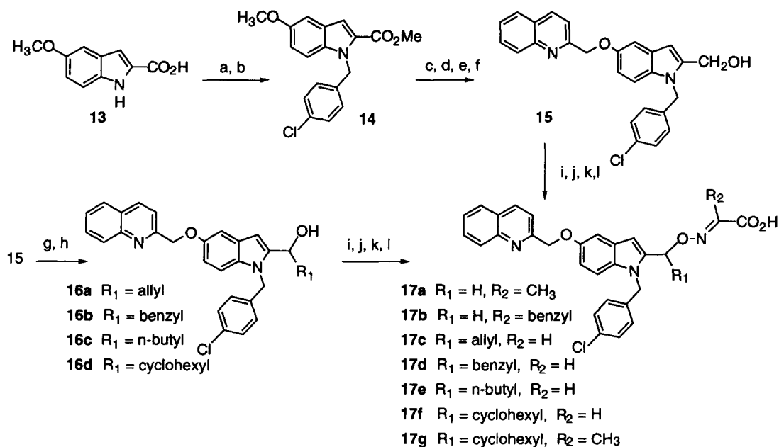
Scheme 3. Reagents: (a) MeI, NaHCO 3 , DMF (69%); (b) p -ClBzCl, NaH, DMF (94%); (c) AlCl 3 , t -BuSH, CH 2 Cl 2 (97%); (d) 2-chloromethylquinoline, K 2 CO 3 , DMF (64%); (e) NaOH, dioxane, MeOH (95%); (f) ClCO 2 Et, Et 3 N, THF, -15 °C, then NaBH 4 , MeOH, 0 °C (93%); (g) Ba(MnO 4 ) 2 , toluene, reflux (88%); (h) RMgX, THF, -78 °C; (i) PhNOH, Ph 3 P, DEAD, THF; (j) H 2 NNH 2 , dioxane, EtOH; (k) CH 3 COCO 2 CH 3 , AcOH, dioxane, methanol; (l) NaOH, dioxane, MeOH. Overall yield from 15 : 17a (10%), 17b (4%), 17c (15%), 17d (13%), 17e (35%), 17f (9%), and 17g (11%).
